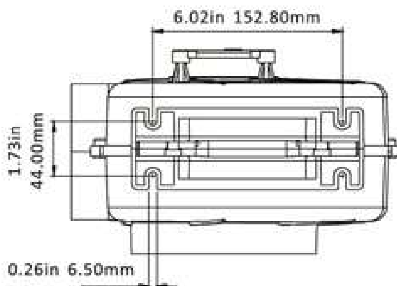
Flex Mount-02
