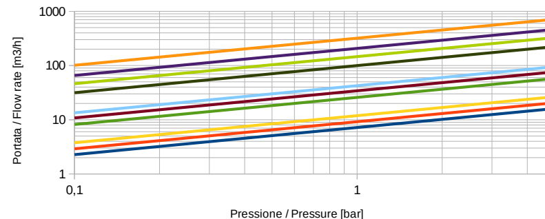
Filtro Acqua - Water Strainer Art. 0005 / 2005 / 7005 "GENOVA"
